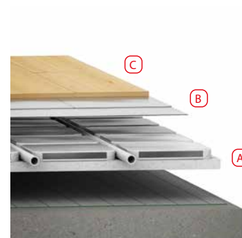
Section with R881XPS panel
